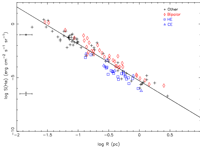
Figure 2. Newly derived H\alpha surface brightness – radius relation based on a large sample of calibrating PNe. Bipolars (red diamonds) are seen to be larger, and hence more massive, at a given surface brightness. Common-envelope (CE) PNe (blue triangles) have systematically lower masses and define a separate trend in SB-r space, coincident with high excitation (HE) PNe (blue squares). Other calibrating PNe are marked with crosses. The line is a linear least-squares fit to the entire sample, and representative errors bars are shown.
