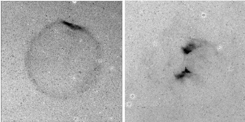
Figure 1. Continuum-subtracted H\alpha images of PFP 1 (Pierce et al. 2004) and RCW 24 (Frew, Parker & Russeil 2006), two large evolved PNe in the Solar Neighbourhood. Both images are 30 arcmin wide.
