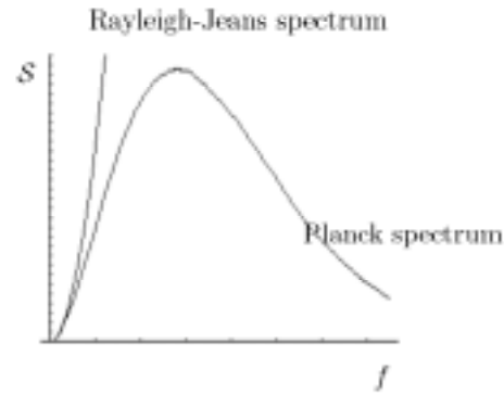
Figure 2.1: Rayleigh-Jeans (classical) and Planck spectral distributions.
